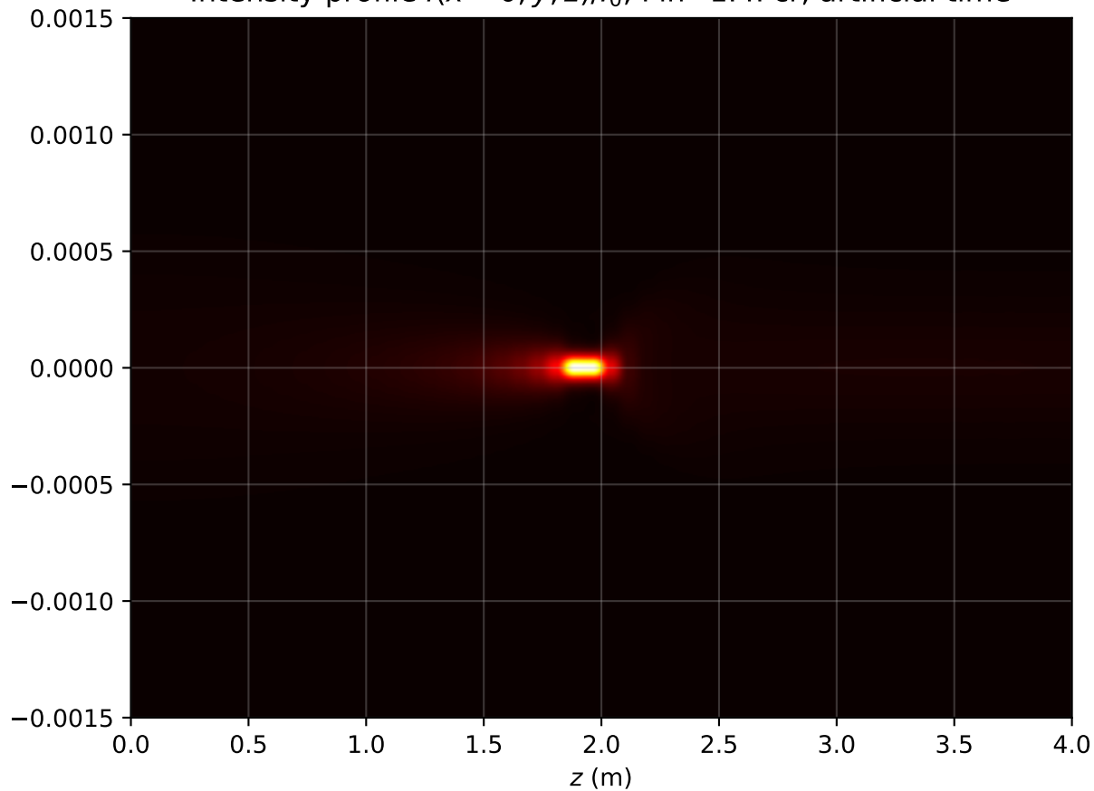
Intensity profile I(x=0, y, z)/I_0 , P_{in}=1.4P_{cr} , artificial time
